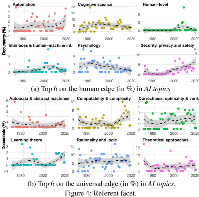
Figure 4: Referent facet.
